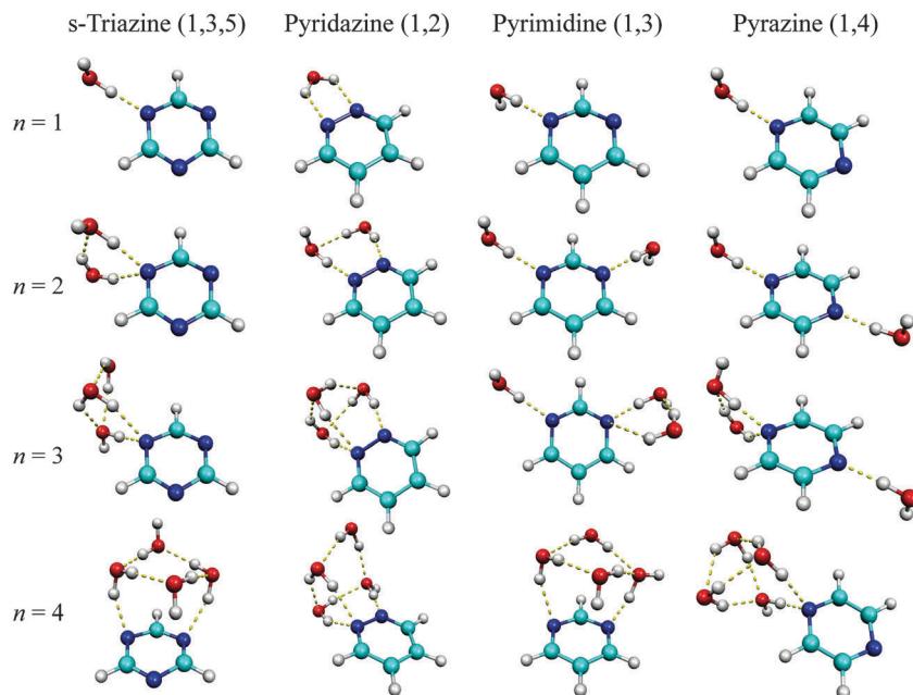
Fig. 4 Lowest energy structures of \text{Tz}^- \cdot (\text{H}_2\text{O})_n , \text{Pd}^- \cdot (\text{H}_2\text{O})_n , \text{Pm}^- \cdot (\text{H}_2\text{O})_n , and \text{Pz}^- \cdot (\text{H}_2\text{O})_n cluster anions for n = 1-4 using M06-2X/6-31++G(d,p) level of theory.
